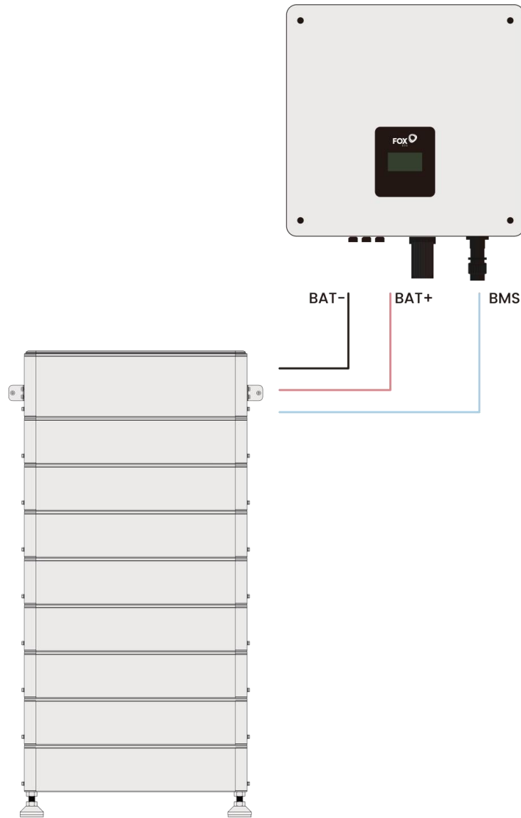
System diagram
